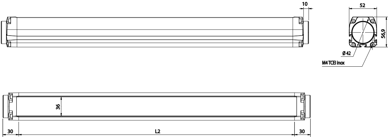
Passive part – All dimensions in mm
