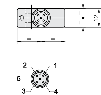
Adam M12-5 male connector. (Note that some models have 4 or 8 pins instead.)
